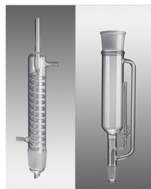
EXTRACTION APPARATUS with coil condenser and ground glass joints BORO 3.3
