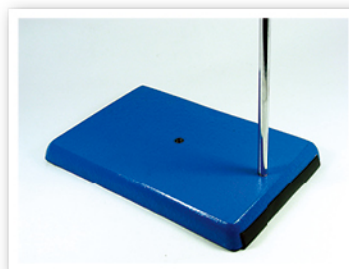
英式铁铸方台 Rectangular Retort Stand Base Cast iron, with hole tapped M10×1.5mm and rubber feet in the short side.
